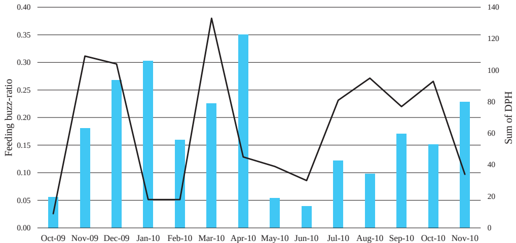
Figure 2. Feeding buzz-ratios (FBR) per month (blue bars) versus acoustic activity expressed as the summation of detection positive hours (DPH) per month (black line) for C-POD location GSP03.
