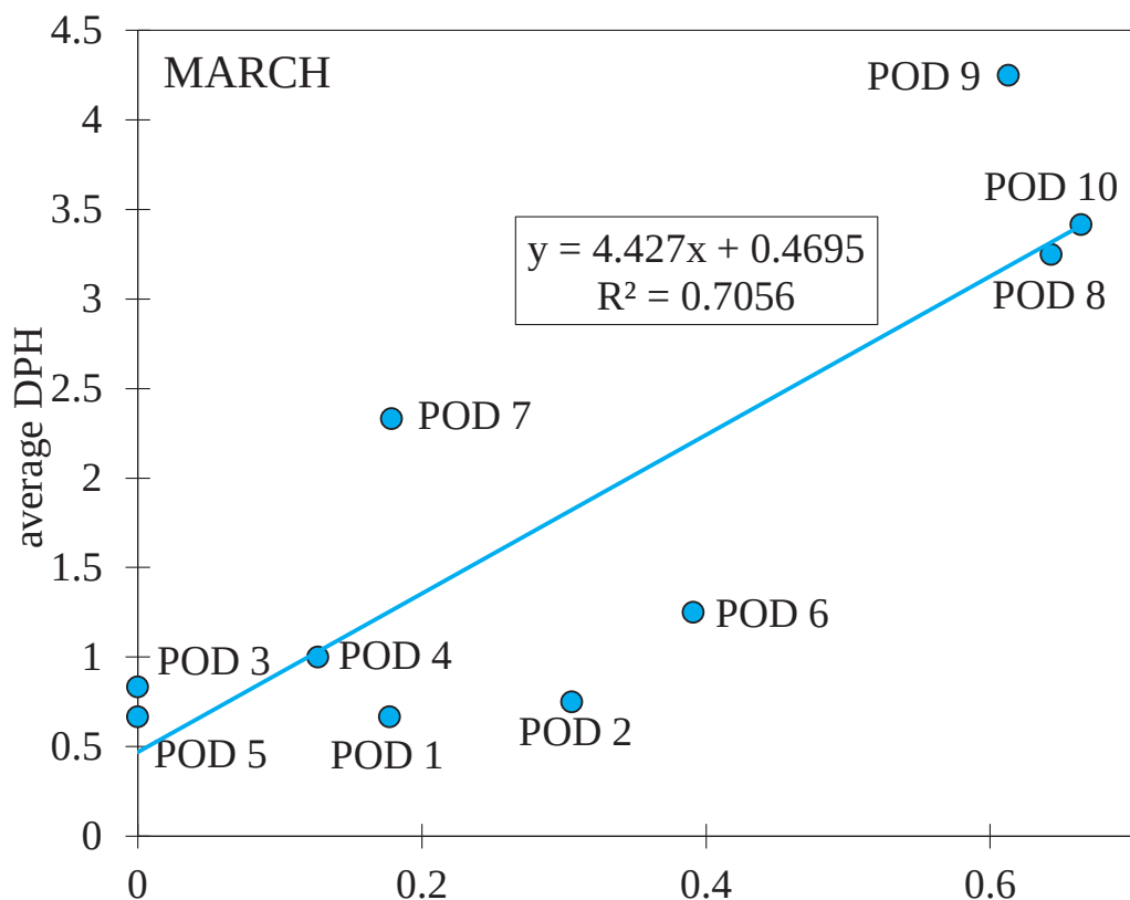
Figure 4. Scatter plot showing average detection positive hours (DPH) and feeding buzz ratio (FBR) per C-POD station (POD 1 to POD 10) for March 2010.
